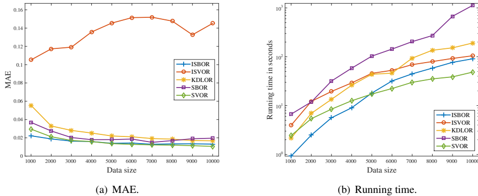
Figure 2: MAE and running time of OR algorithms on the synthetic dataset.
