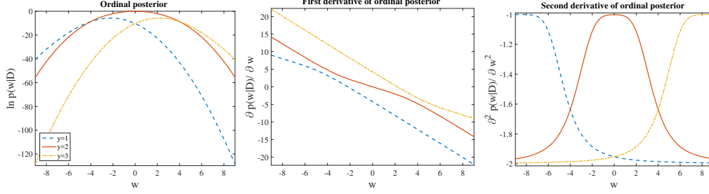
Figure 1: The ordinal posterior and its first and second derivatives.
